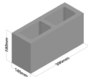
Hollow 150 390*190*140mm
